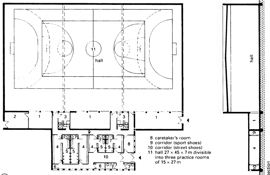
2 Plan layout of a triple sports hall
